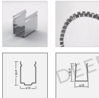
MOUNTING CLIPS CURVED ALUMINUM PROFILE
